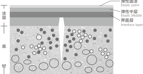
弹性涂层的抗开裂 Cracking resistance of elastomeric coating
